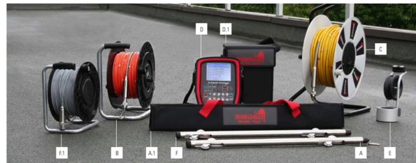
A Digital inclinometer probe A.1 Travel bag for both inclinometer and dummy probes B Light inclinometer cable reel C Heavy-Duty cable D Archimede readout D.1 Archimede carrying case E Pulley assembly F Dummy probe F.1 Cable for dummy probe
